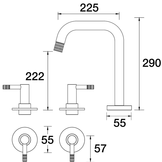
Elm Lane Sink Set Hob Swivel B42.051.1.40 - Rumbled Brass
