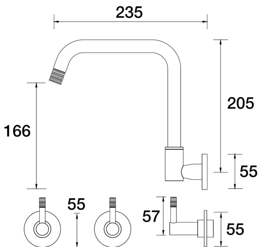
Elm Lane Sink Set Wall Swivel B42.052.1.02 - Brushed Chrome
