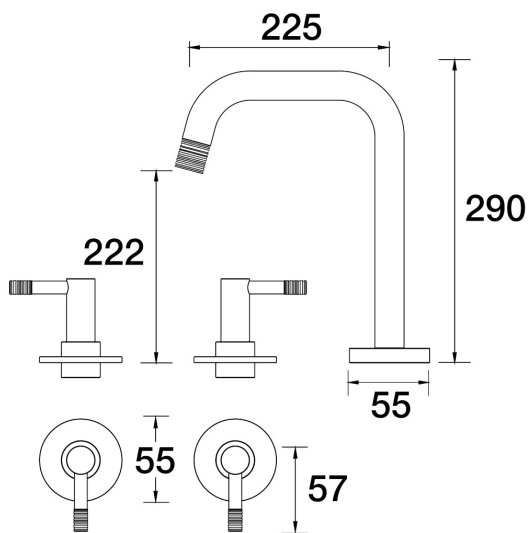
Elm Lane Spa Set Hob Swivel B42.061.1.48 - Copper
