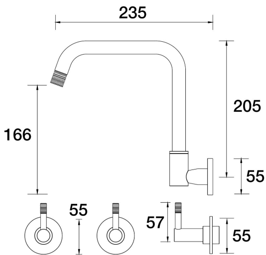
Elm Lane Spa Set Wall Swivel B42.062.1.12 - 23k Brushed Gold
