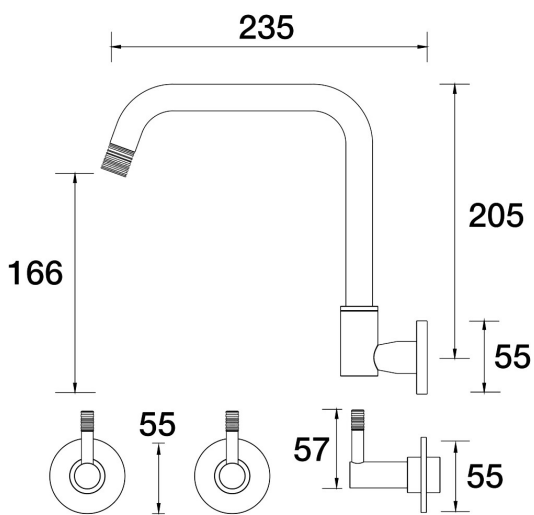
Elm Lane Spa Set Wall Swivel B42.062.1.54 - Volcanic Grey
