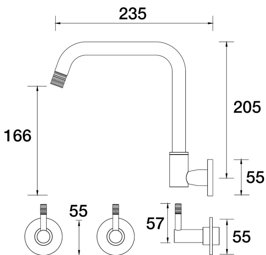
Elm Lane Spa Set Wall Swivel B42.062.1.67 - Vintage Brass
