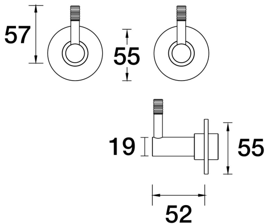
Elm Lane Top Assemblies Wall Pair B42.082.1.43 - Brass
