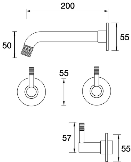
Elm Lane Wall Basin Set 200mm Outlet B42.152.1.43 - Brass
