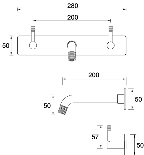
Elm Lane Wall Basin Set 200mm Outlet On Plate B42.152.2.11 - 23k Gold
