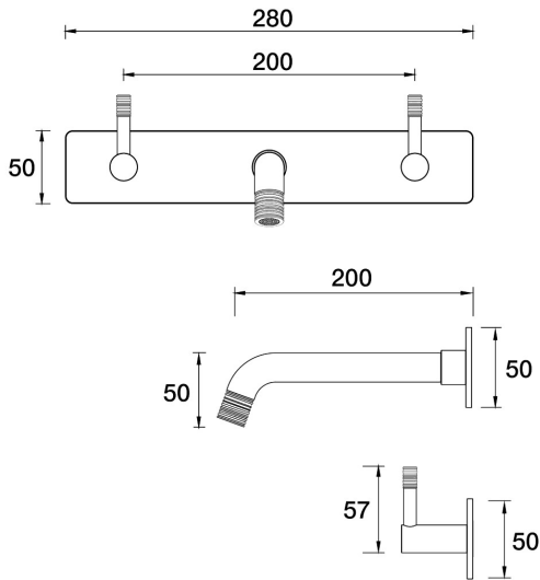
Elm Lane Wall Basin Set 200mm Outlet On Plate B42.152.2.57 - Matt Nickel
