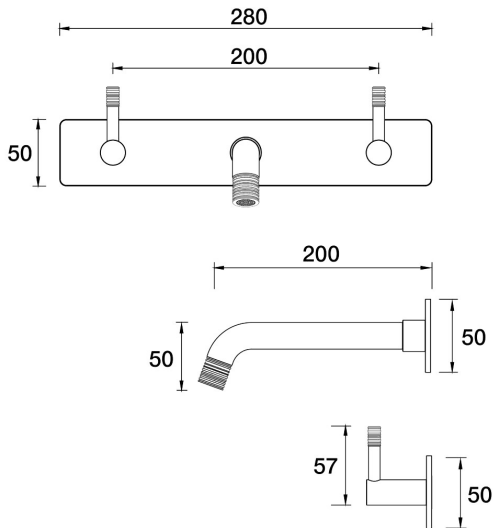
Elm Lane Wall Basin Set 200mm Outlet On Plate B42.152.2.68 - Autumn Bronze
