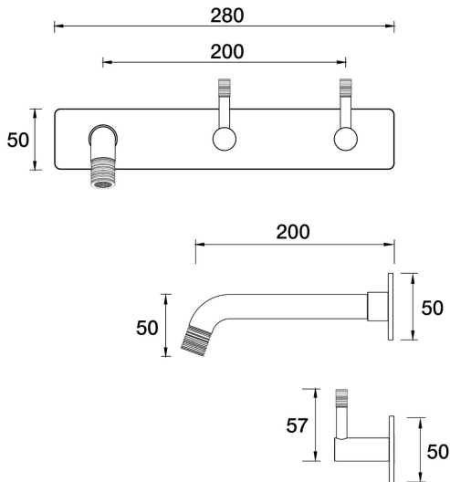
Elm Lane Wall Basin Set 200mm Outlet On Plate - Offset
