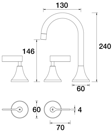
ARI Basin Set Swivel Lever Ceramic Disc B43.011.3.01 - Chrome
