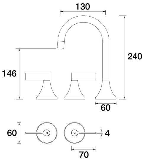
ARI Basin Set Swivel Lever Ceramic Disc B43.011.3.27 - Satin Pearl
