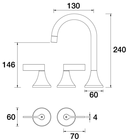
ARI Basin Set Swivel Lever Ceramic Disc B43.011.3.52 - Burnished
