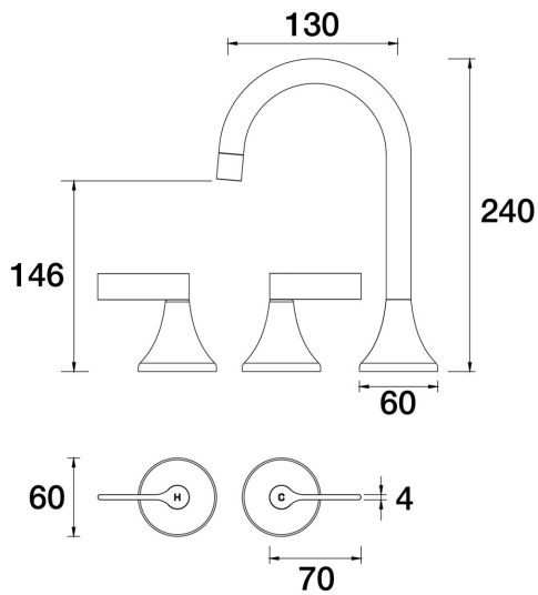
ARI Basin Set Swivel Lever Ceramic Disc B43.011.3.67 - Vintage Brass
