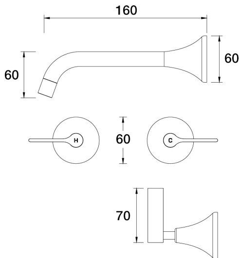
ARI Wall Bath Set 160mm Outlet Lever Ceramic Disc Dec 2021.3.02 - Brushed Chrome
