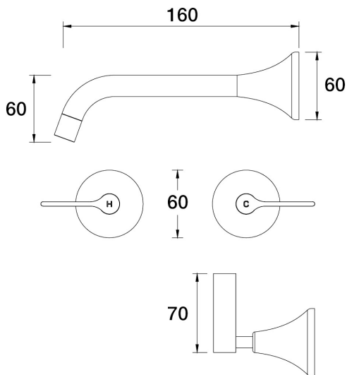
ARI Wall Bath Set 160mm Outlet Lever Ceramic Disc Part No. 21.3.48 - Copper
