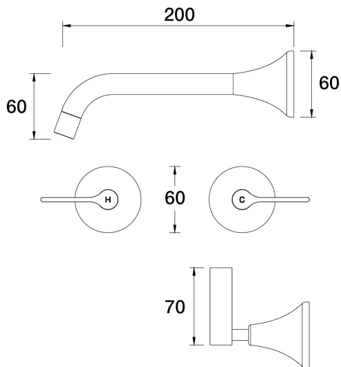
ARI Wall Bath Set 200mm Outlet Lever Ceramic Disc Part No. 2022.3.43 - Brass
