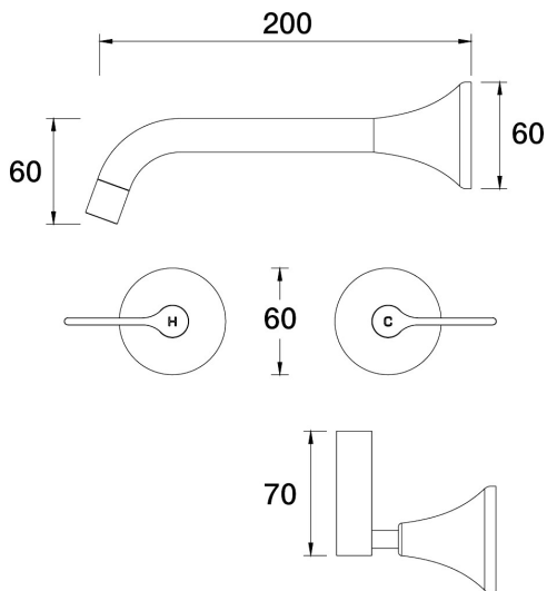
ARI Wall Bath Set 200mm Outlet Lever Ceramic Disc Part No. 22.3.48 - Copper
