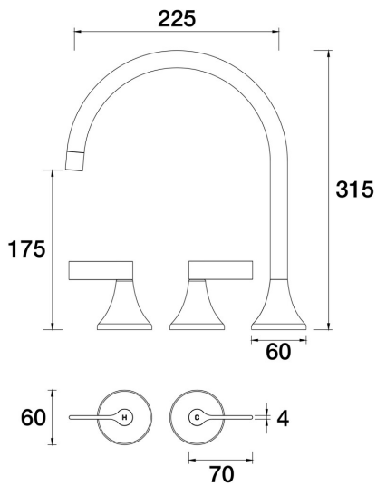
ARI Sink Set Hob Swivel Lever Ceramic Disc B43.051.3.67 - Vintage Brass
