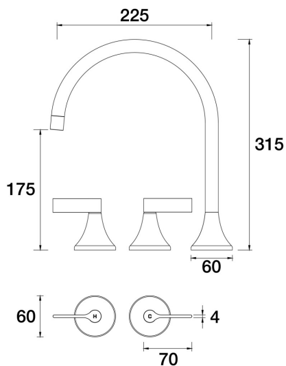
ARI Spa Set Hob Swivel Lever Ceramic Disc B43.061.3.25 - Brushed Nickel
