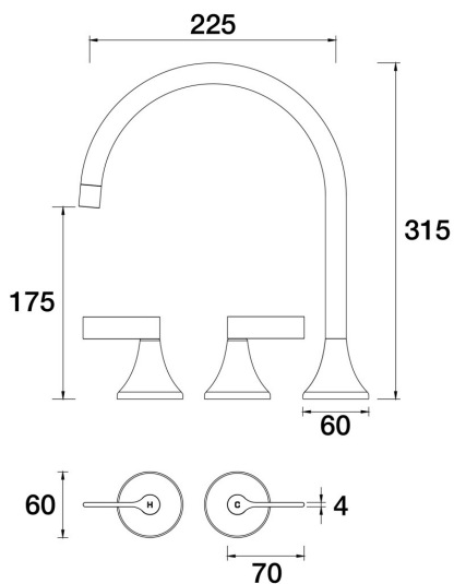
ARI Spa Set Hob Swivel Lever Ceramic Disc B43.061.3.42 - Brushed Copper
