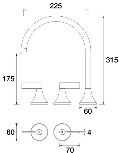
ARI Spa Set Hob Swivel Lever Ceramic Disc B43.061.3.43 - Brass
