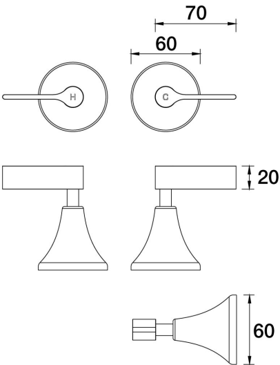
ARI Top Assemblies Wall Pair Lever Ceramic Disc B43.082.3.01 - Chrome
