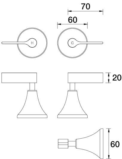
ARI Top Assemblies Wall Pair Lever Ceramic Disc B43.082.3.23 - Gunmetal
