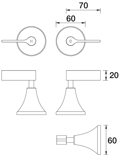
ARI Top Assemblies Wall Pair Lever Ceramic Disc B43.082.3.54 - Volcanic Grey
