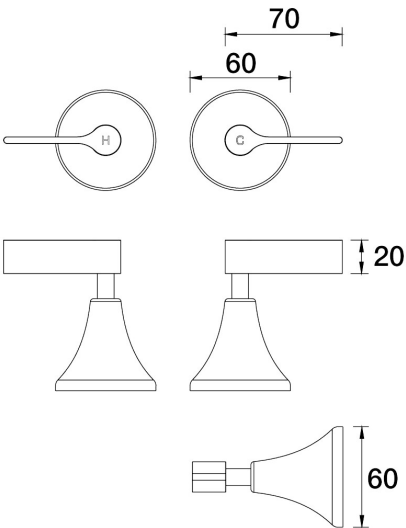
ARI Top Assemblies Wall Pair Lever Ceramic Disc B43.082.3.67 - Vintage Brass
