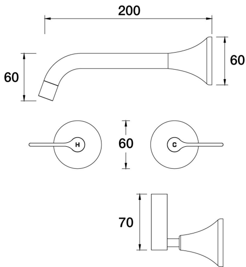
ARI Wall Basin Set 200mm Outlet Lever Ceramic Disc B43.152.3.01 - Chrome
