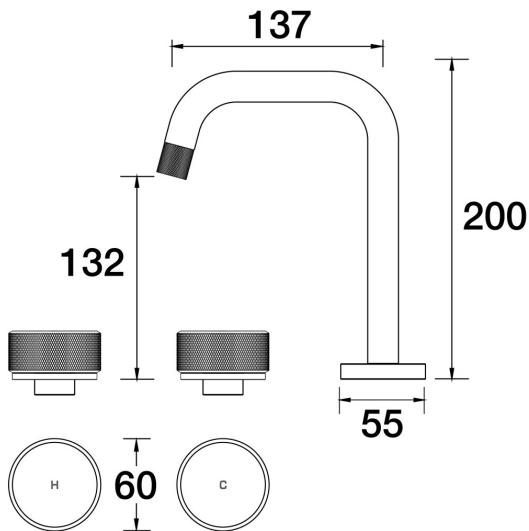
Opus Basin Set Basin Set Swivel B45.011.1.21 - Brushed Rose Gold
