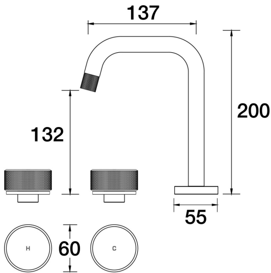
Opus Basin Set Basin Set Swivel B45.011.1.23 - Gunmetal
