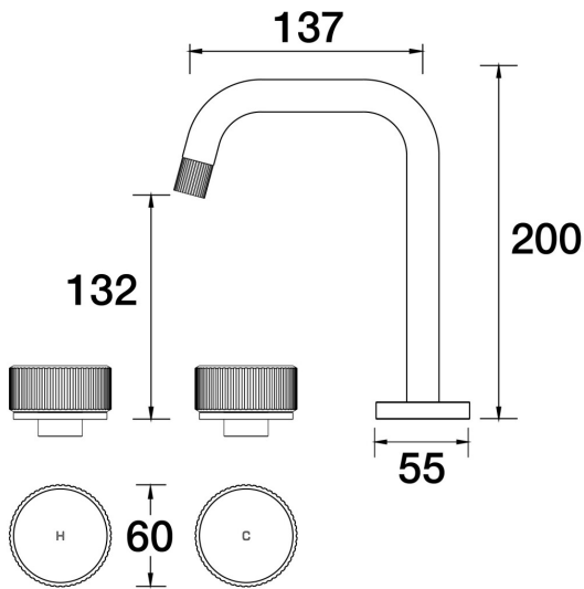
Opus Basin Set Basin Set Swivel Lane B45.011.2.01 - Chrome
