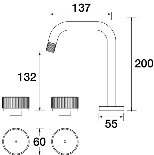
Opus Basin Set Basin Set Swivel Lane B45.011.2.27 - Satin Pearl
