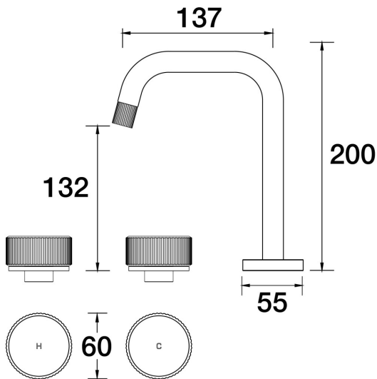
Opus Basin Set Basin Set Swivel Lane B45.011.2.48 - Copper
