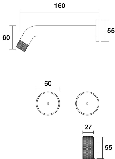
Opus Wall Bath Set Bath Set 160mm Outlet B45.021.1.01 - Chrome
