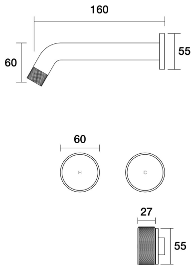
Opus Wall Bath Set 160mm B45.021.1.34 - Matt Black
