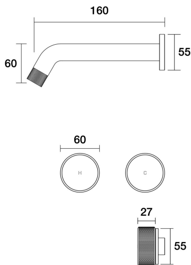
Opus Wall Bath Set 160mm B45.021.1.45 - Native Brass
