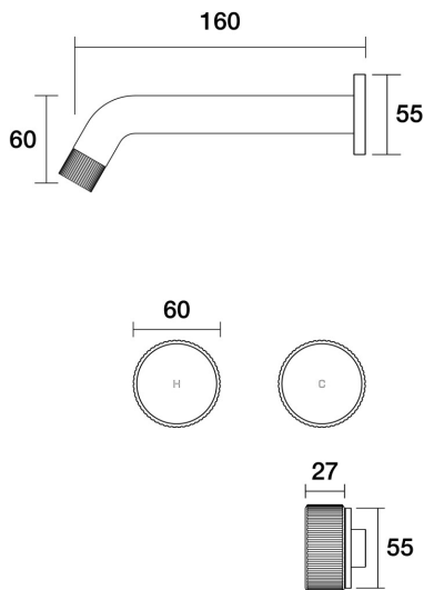
Opus Wall Bath Set 160mm Lane B45.021.2.11 - 23k Gold
