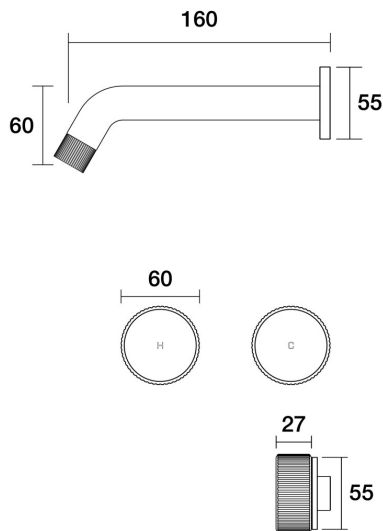
Opus Wall Bath Set 160mm Lane B45.021.2.40 - Rumbled Brass
