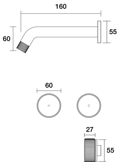
Opus Wall Bath Set 160mm Lane B45.021.2.41 - Brushed Brass
