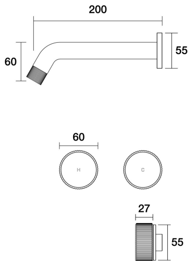
Opus Wall Bath Set 200mm Lane B45.022.2.34 - Matt Black
