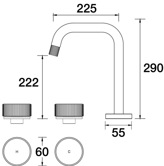
Opus Sink Set Hob Swivel Lane B45.051.2.34 - Matt Black
