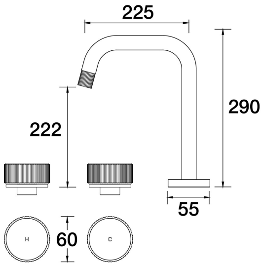
Opus Sink Set Hob Swivel Lane B45.051.2.57 - Matt Nickel
