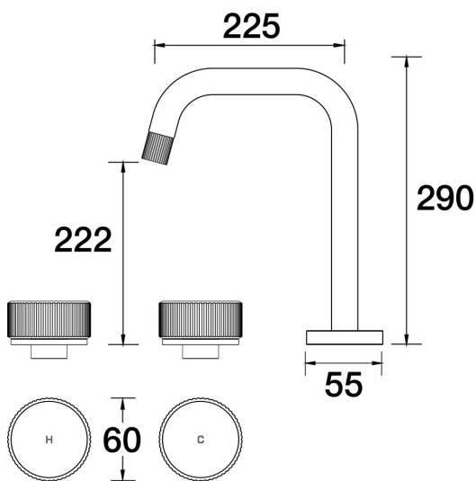
Opus Sink Set Hob Swivel Lane B45.051.2.67 - Vintage Brass
