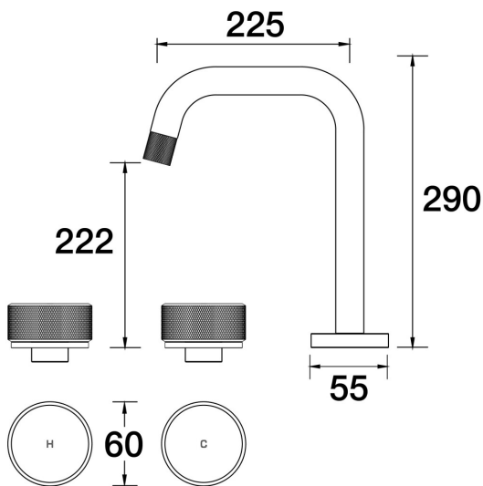
Opus Spa Set Hob Swivel B45.061.1.47 - Luminick
