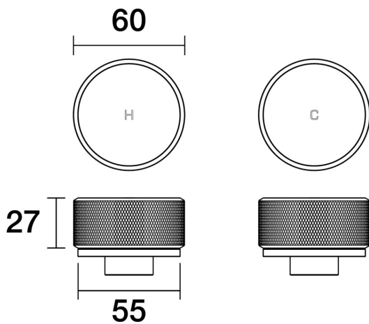
Opus Top Assemblies Pair B45.082.1.12 - 23k Brushed Gold
