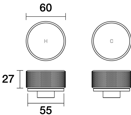
Opus Top Assemblies Pair B45.082.1.44 - Antique Copper
