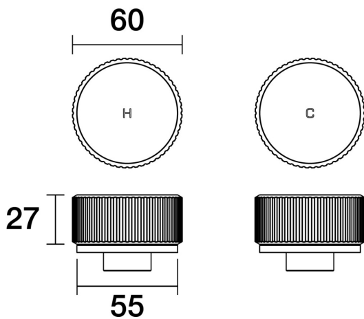
Opus Top Assemblies Pair Lane B45.082.2.01 - Chrome
