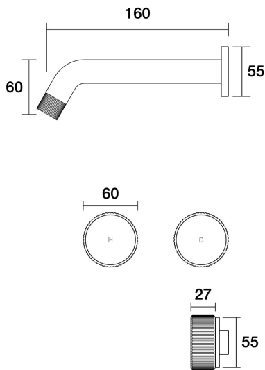
Opus Wall Basin Set 160mm Outlet Lane B45.151.2.43 - Brass
