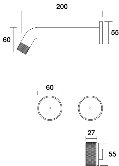
Opus Wall Basin Set 200mm Outlet B45.152.1.02 - Brushed Chrome
